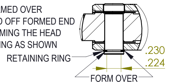
DETAIL A SCALE 1.5 : 1 DEFORM BEFORE CALIBRATION
